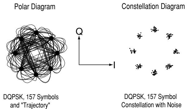
Figure 26. Constellation Diagram
