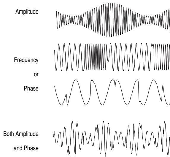
Figure 4. Signal Characteristics to Modify
